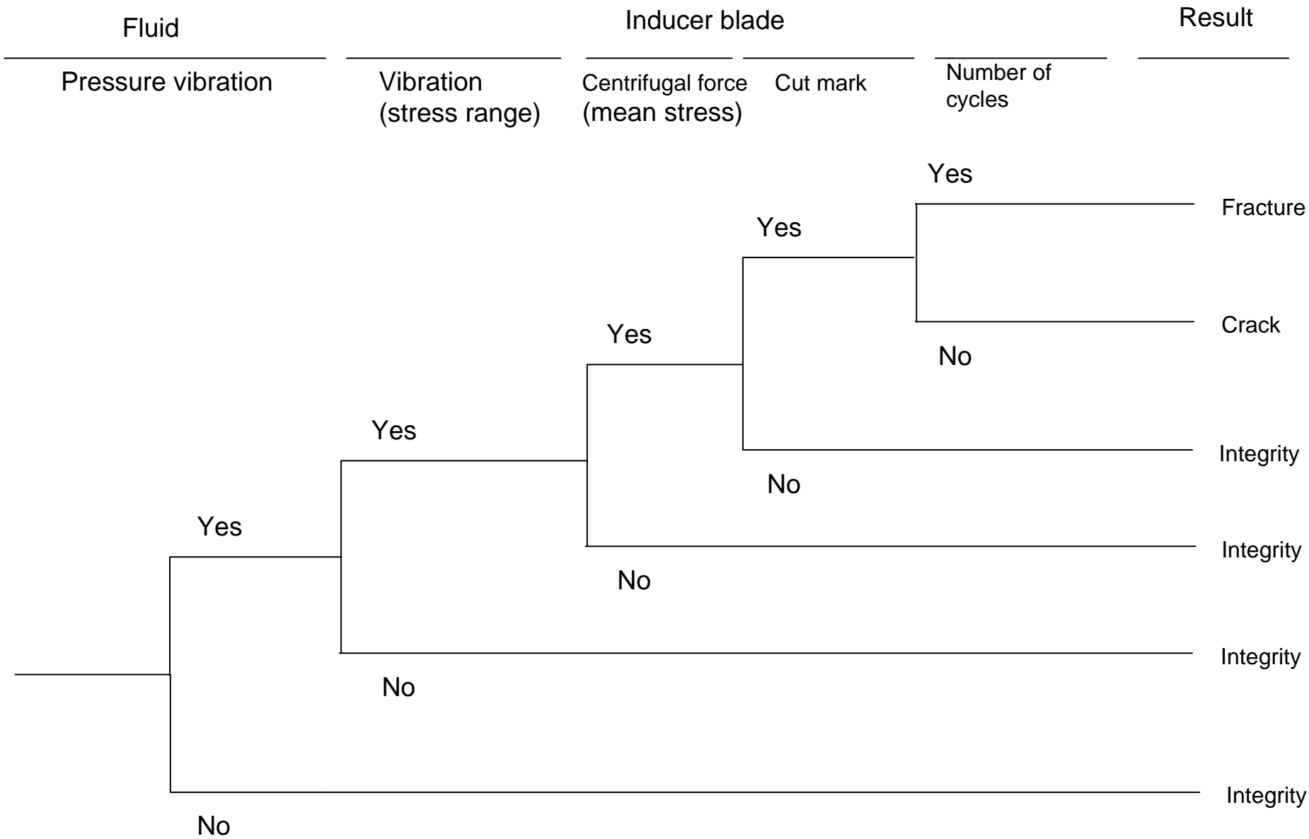
Fig.5 Event tree diagram for the inducer blade fatigue fracture caused by vibration
